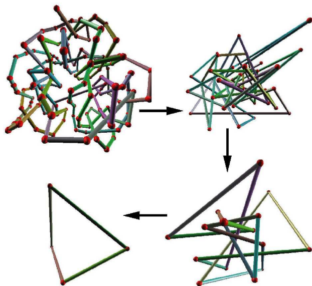
Figure 7.31: The planner in [89] untangles the famous Ochiai unknot benchmark in a few minutes on a standard PC.
