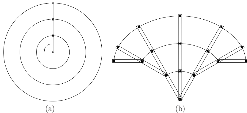
Figure 7.26: (a) If any joint angle is possible, then the links sweep out a circle in the limit. (b) If there are limits on the joint angles, then a tighter bound can be obtained for the reachability of the linkage.
