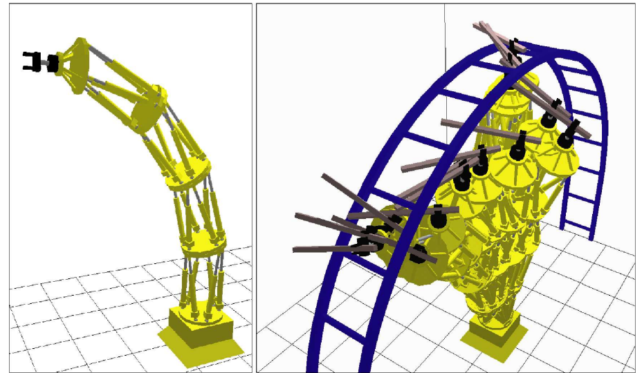
Figure 7.27: Planning for the Logabex LX4 robot [31]. This solution was computed in less than a minute by applying active-passive decomposition to an RDT-based planner [41]. In this example, the dimension of \mathcal{C} is 97 and the dimension of \mathcal{C}_{do} is 25.
