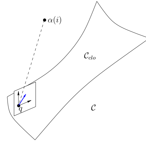
Figure 7.22: For each sample \alpha(i) the nearest point, q_n \in \mathcal{C} , is found, and then the local planner generates a motion that lies in the local tangent plane. The motion is the project of the vector from q_n to \alpha(i) onto the tangent plane.
