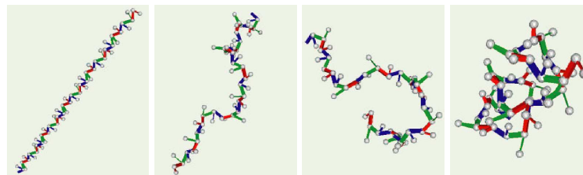
Figure 7.34: Protein folding for a polypeptide, computed by a sampling-based roadmap planning algorithm [10]
