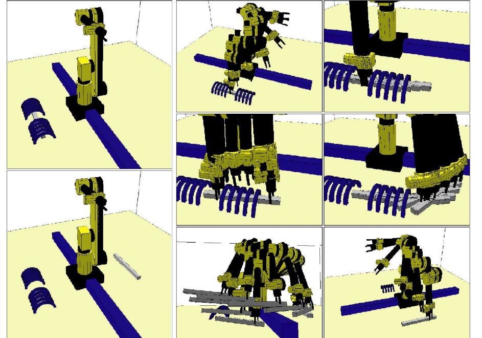
Figure 7.17: This example was solved in [41] using the manipulation planning framework and the visibility-based roadmap planner. It is very challenging because the same part must be regrasped in many places.
