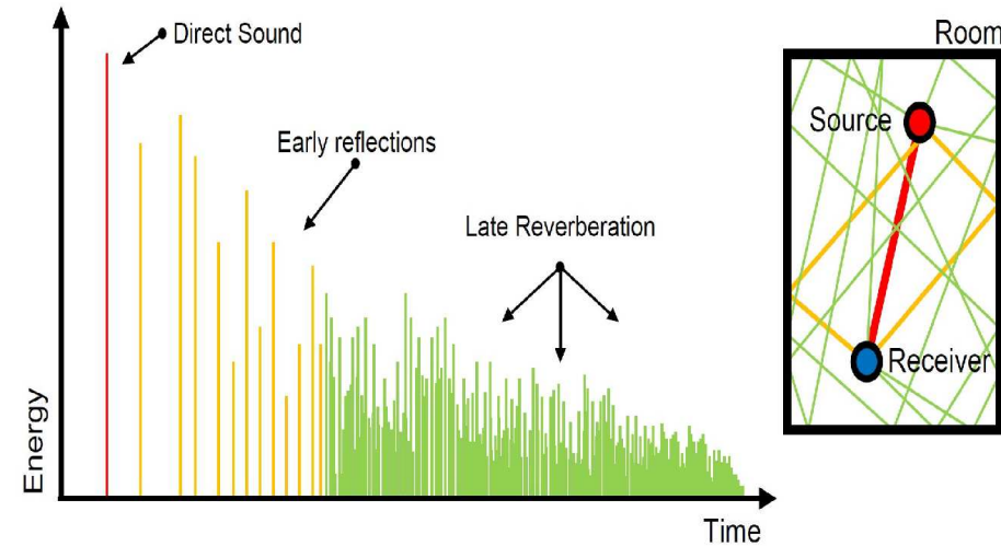
Figure 11.15: Reverberations. (From Pelzer, Aspöck, Schroder, and Vorländer, 2014, [253])
