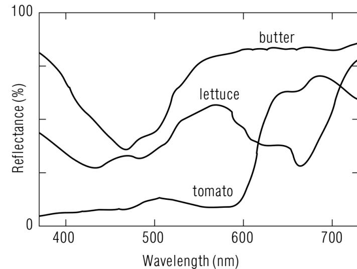
Figure 4.7: The spectral reflection function of some common familiar materials. (Figure from [298]).
