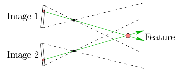
Figure 9.27: By using two cameras, stereo vision enables the location of a feature in the 3D world to be determined by intersecting the corresponding visibility ray from each camera. To accomplish this, the camera calibration parameters and relative poses must be known. Similarly, one camera could be replaced by a laser that illuminates the feature so that it is visible to the remaining camera. In either case, the principle is to intersect two visibility rays to obtain the result.
