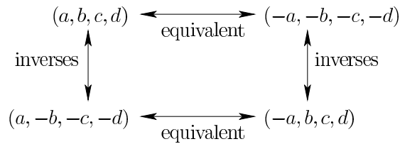
Figure 3.12: Simple relationships between equivalent quaternions and their inverses.
