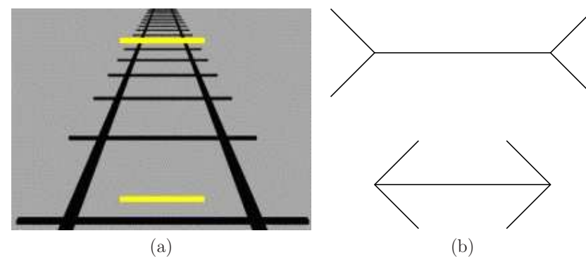
Figure 6.2: Even simple line drawings provide significant cues. (a) The Ponzo illusion: The upper yellow bar appears to be longer, but both are the same length. (b) The Müller-Lyer illusion: The lower horizontal segment appears to be shorter than the one above, but they are the same length.
