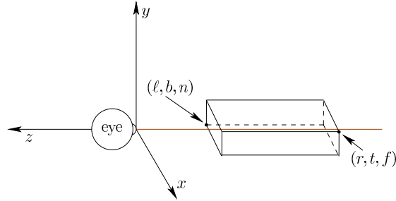
Figure 3.19: The rectangular region formed by the corners of the viewing frustum, after they are transformed by T_p . The coordinates of the selected opposite corners provide the six parameters, \ell , r , b , t , n , and f , which are used in T_{st} .
