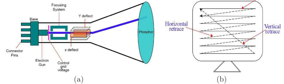
Figure 4.35: (a) In a cathode ray tube (CRT), an electron gun emits a beam of electrons, which are deflected in both X and Y directions according to an analog signal. When the beam hits the screen, an element of phosphor briefly lights up. (b) A special scanning pattern was used to draw out each video frame, line by line.
