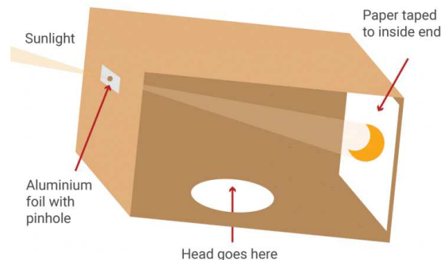
Figure 4.31: A pinhole camera that is recommended for viewing a solar eclipse. (Figure from from https://www.timeanddate.com/. )
