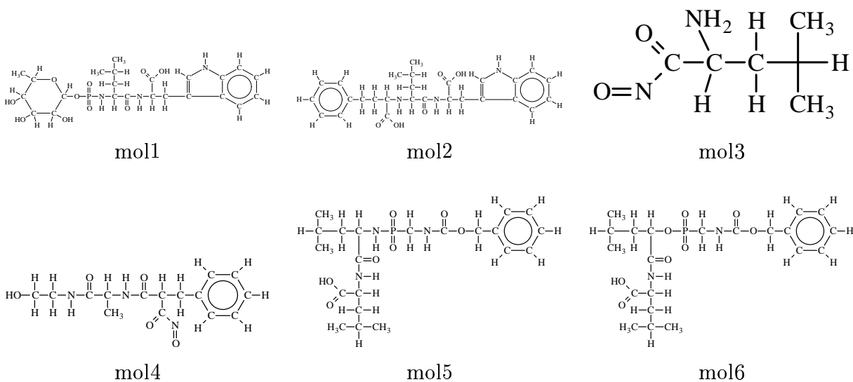
Figure 9: The inhibitors of thermolysin used in our experiments.
